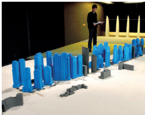
Figure 8.1 Wind tunnel testing Courtesy of BMT Fluid Dynamics
