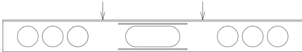
Figure 4.5 – Cellular beam solution with central elongated opening
