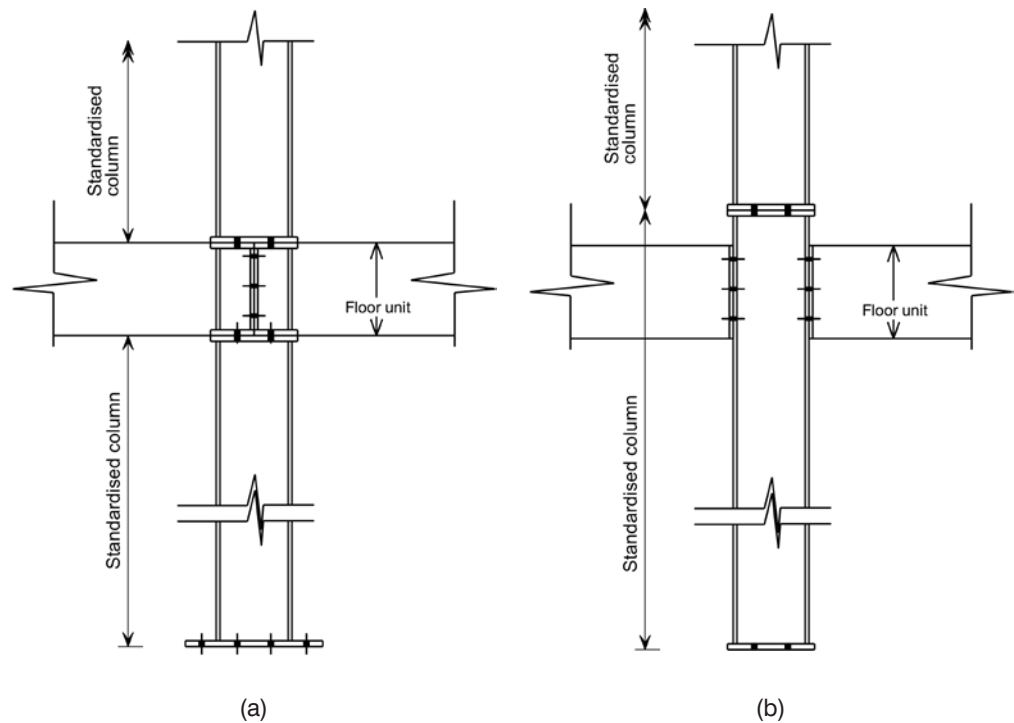
Figure 3.4 - Single storey column arrangements
