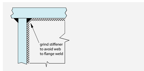
Figure 6 Alternative stiffener detail at corner
