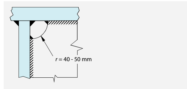
Figure 5 Cope hole detail
